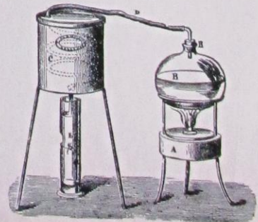
WINE STILL
