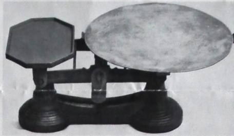
No. II.—SCALE PLATE BY SAMUEL COCKS WITH PLAIN SIDE UP IN ACTUAL USE CIRCA 1820
